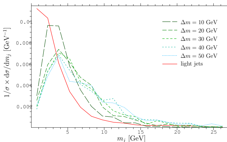
Figure 5: Jet mass distribution for charm jets from stop decays for different \Delta m , compared to light flavor jets from ISR.
