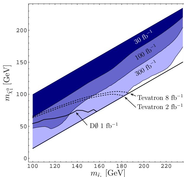
Figure 3: Projected LHC 5\sigma discovery reach in the jet+ \cancel{E}_T channel. For comparison the current and future Tevatron 95% C.L. exclusion bounds for light stops are also shown.
