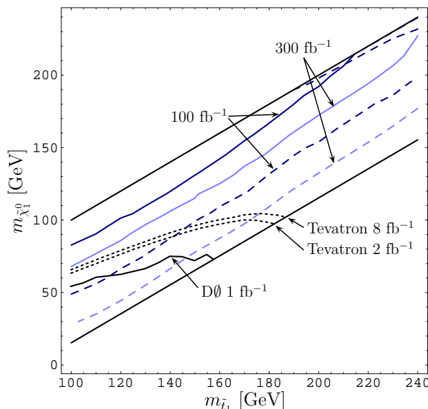
Figure 6: Improvement of projected LHC reach in the \gamma + \cancel{E}_T channel from charm tagging, for 100\text{ fb}^{-1} (dark lines) and 300\text{ fb}^{-1} (light lines). The solid lines correspond to the right side of figure 2 which has no charm tagging, while the dashed lines indicate the extended reach due to charm tagging as described in the text.
