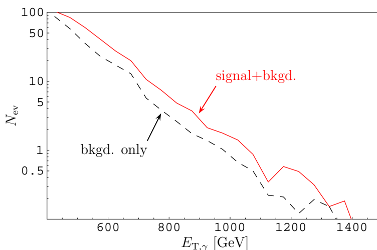
Figure 1: Distribution of the photon transverse energy, E_{T,\gamma} , for the SM background (from ref. [27]) and the stop signal with m_{\tilde{t}_1}=130 \text{ GeV} and m_{\tilde{\chi}_1^0}=110 \text{ GeV} . The fluctuations at the right end of the plot are due to Monte Carlo errors.
